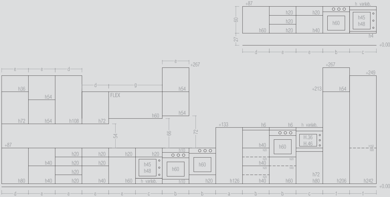
MODULARITA' BASI SOSPESI: vista frontale. WALL-MOUNTED BASE CABINETS MODULARITY: front view.
