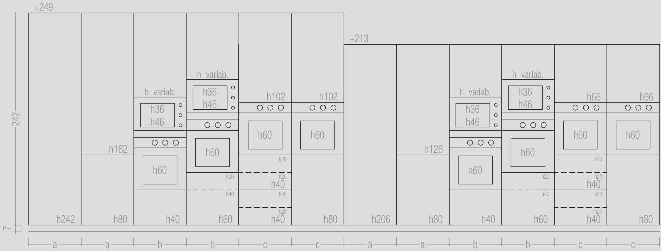
MODULARITA' BASI, PENSILI, ARMADI, COLONNE: vista frontale. BASE CABINETS, WALL CABINETS, TALL UNITS & CUPBOARDS MODULARITY: front view.
