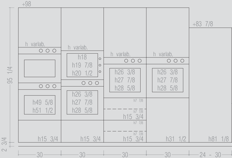
BASE CABINETS AND TALL UNITS MODULARITY for US standard appliances: front view.
