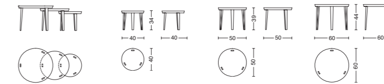
Cod. TAO SMALL Ø 40 - H. 34
